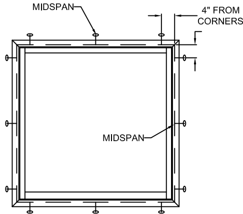
TYPICAL ELEVATION WITH FASTENER SPACING
