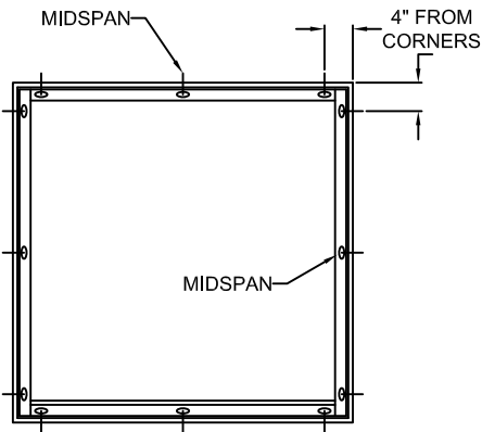
TYPICAL ELEVATION WITH FASTENER SPACING
